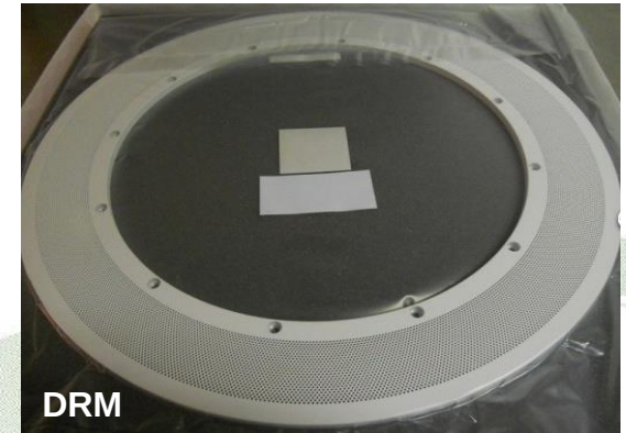
Exhaust Plate, DRM P/n 1D10-100912-11
