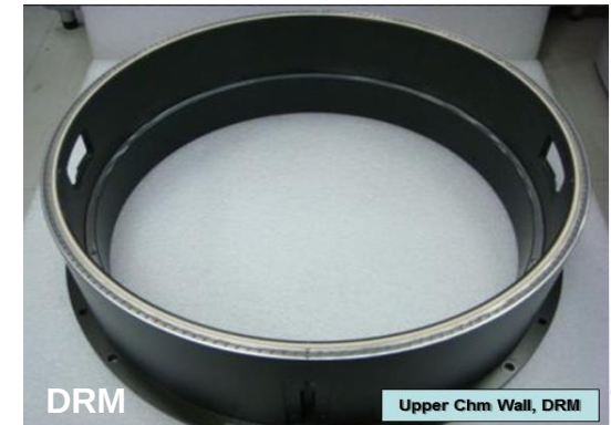
Upper Chamber Wall, DRM
