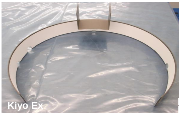
Kiyo Ex Liner Fixed OUTR ACME 2300 P/n 714-045743-809
