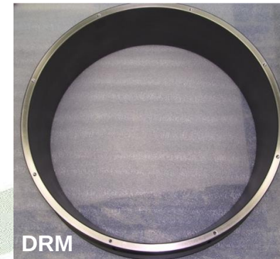
Depo Shield w/o Window (CIP)
