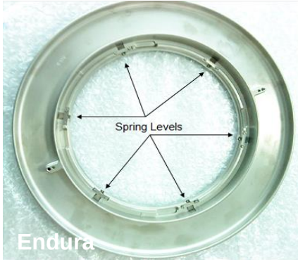
6 Pad Clamp Ring with Spring Lever P/n CT 433-01946-B
