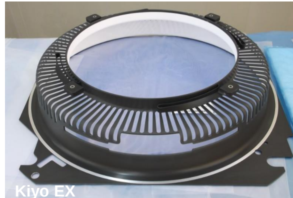
Kiyo EX Liner, Sym Hi Flow, 2300 SRC P/n 715-042721-866
